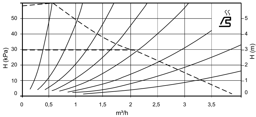
Biral CompAX xx-6 RED / constant \Delta p-c
