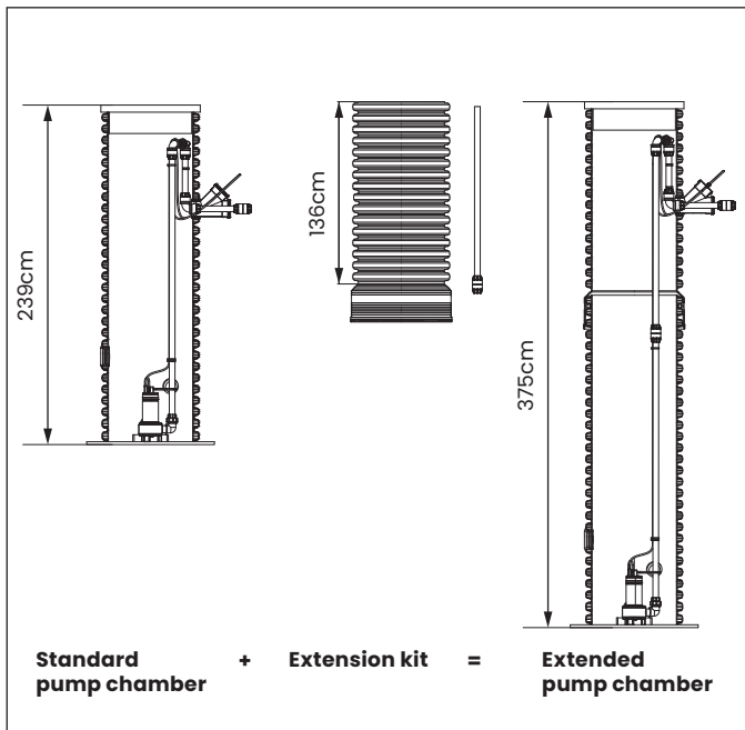
Picture 15 concept with standard height and extension
