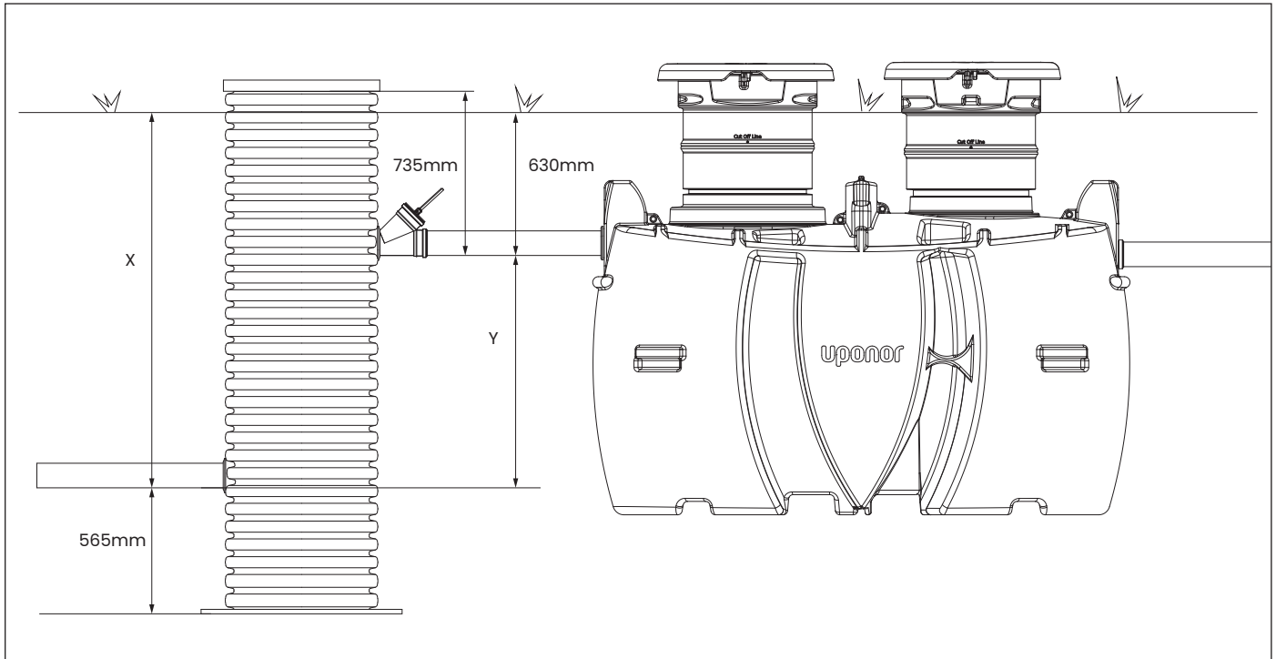
Installation dimensions (Picture 2)
