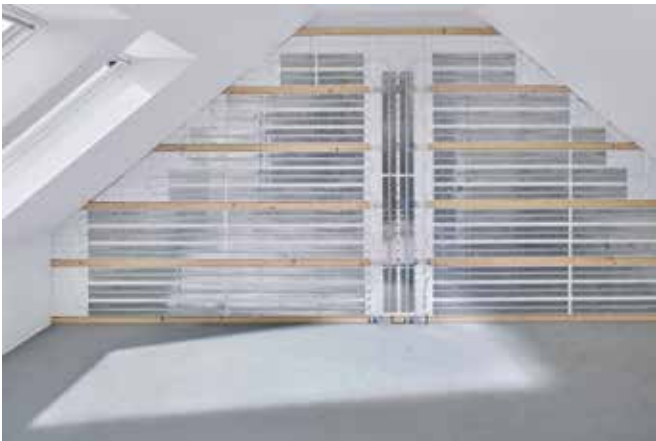
Uponor Siccus plate – laying plate made of EPS with pipe routing channels for holding the Uponor Siccus heat conducting lamellas. Laying spacing 15 / 22.5 / 30 cm.
