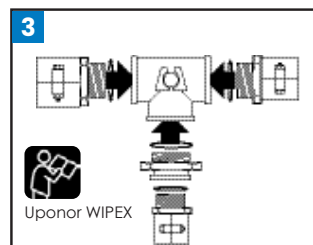
3 Assemble Wipex fittings.
